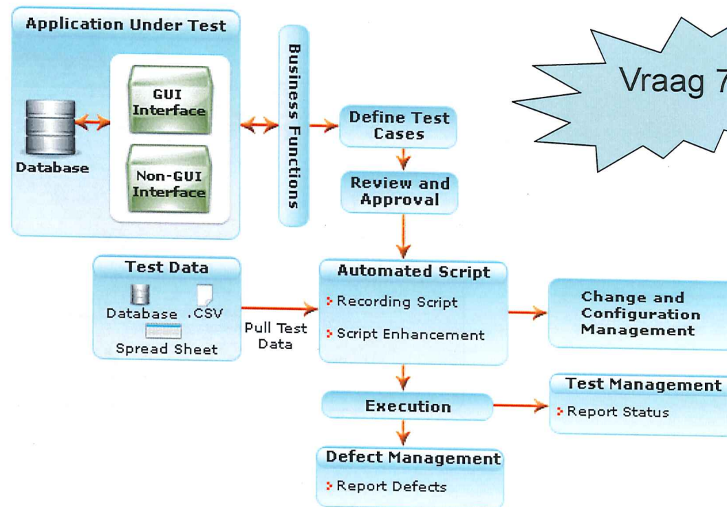
Test Automation Architecture
